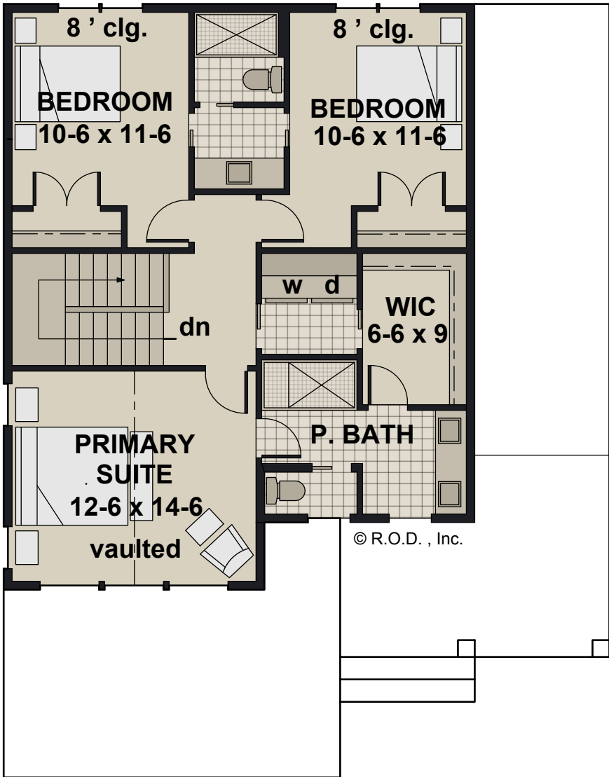
UPPER FLOOR 925 sq. ft.
